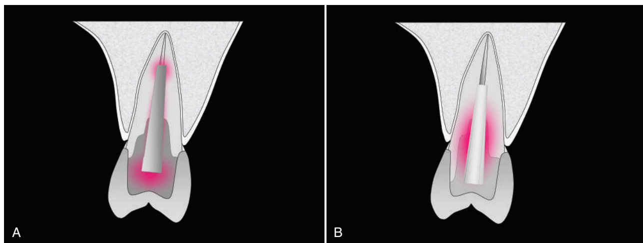
Fig. 23.3 A , Stress distribution within a metallic post and core foundation and residual tooth structure, according to photoelastic studies. The post is cemented and usually penetrates the apical portion of the root. Functional stresses accumulate inside the foundation, slightly around the post and further inside the canal, around the apex of the post; there is less stress buildup in the cervical area compared to that with a fiber post (as shown in Fig. 23.3, B). This configuration more ideally protects the coronocervical structures, but when failing, it results in severe untreatable root fractures. B , Stress distribution within a fiber post/composite foundation and residual tooth structure, according to photoelastic and FEM studies. The post is bonded to the canal walls and penetrates the canal less apically. Functional stresses mainly accumulate around the post in the cervical area. This configuration protects the cervical area less efficiently but tends to prevent untreatable root fractures. The presence of a ferrule is mandatory. (Adapted from Dietschi D, Duc O, Krejci I, Sadan A: Biomechanical considerations for the restoration of endodontically treated teeth: a systematic review of the literature—part 1. Composition and micro- and macrostructure alterations, Quintessence Int 38:733, 2007.)
